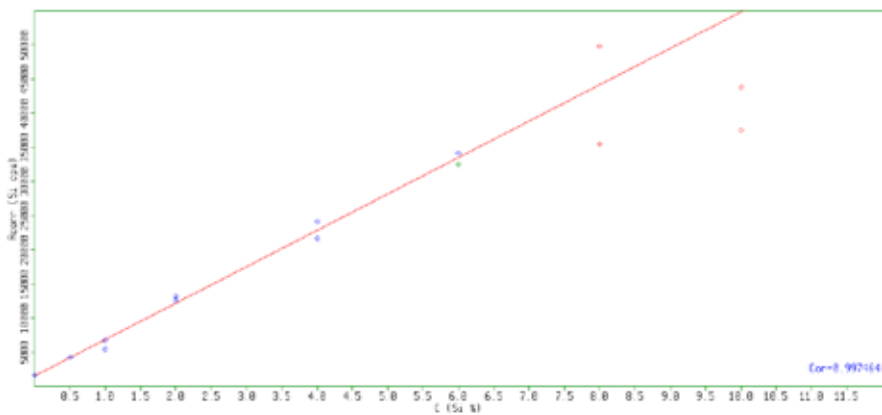
Figure 4. Si Calibration using small pellets. Points highlighted red were excluded
