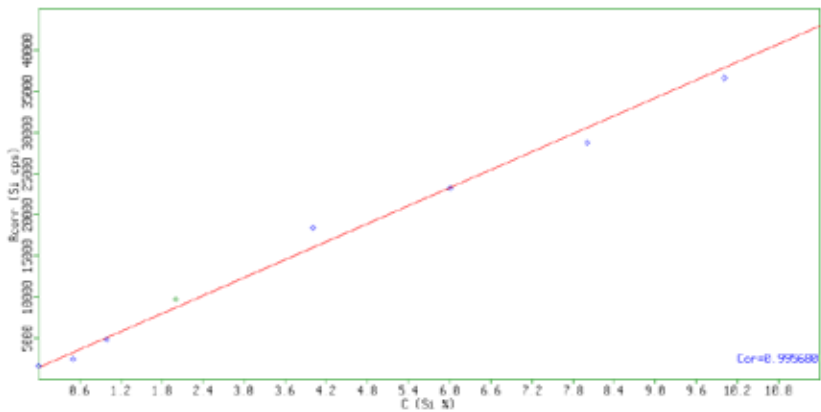
Figure 5. Si Calibration using loose powder in small mass holders
